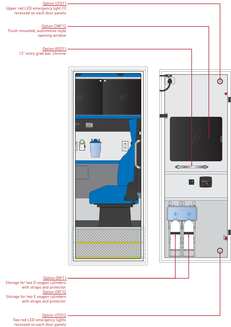
Option CMF12 Access door (C2) with flush-mounted opening window
