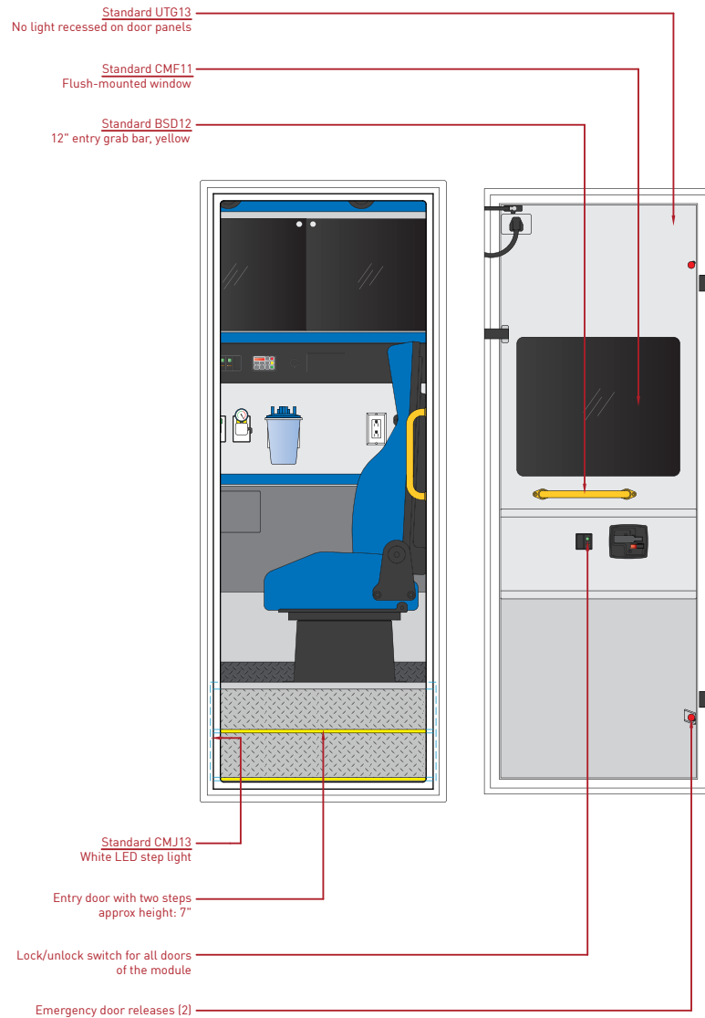
Standard CMF11 Access door (C2) with flush-mounted window
